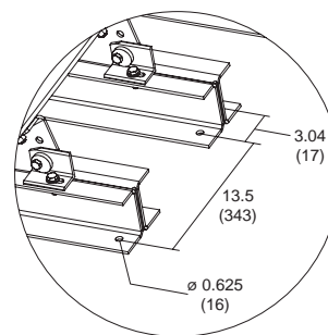
Medium-Duty Cradle
